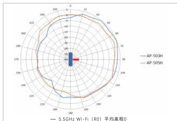
5.5GHz Wi-Fi (天线0, 1)
