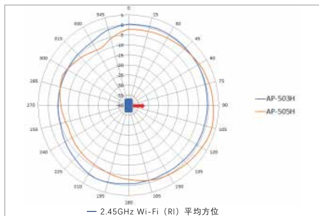
2.45GHz Wi-Fi (天线0, 1)
